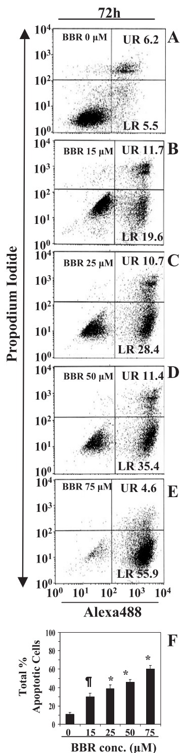
Fig. 4. Berberine induces apoptosis in human epidermoid carcinoma A431 cells in a dose-dependent manner. (A–E), A431 cells were treated with varying concentrations of berberine (0, 15, 25, 50 and 75 μM) in complete medium for 72 h then harvested for the analysis of apoptotic cells by FACS using the Annexin V-Alexa Fluor488 Apoptosis Vybrant Assay Kit following the manufacturer's protocol. The lower right (LR) quadrant of the FACS histograms indicates the percentage of early apoptotic cells (Alexa488-stained cells) and the upper right (UR) quadrant indicates the percentage of late apoptotic cells (Alexa488+propidium iodide-stained cells). (F), Total percent of apoptotic cells in each treatment group was summarized after 72 h of berberine treatment to A431 cells, and data are presented as mean ± SE of three experiments. BBR, berberine. Significant difference versus control group (non-berberine-treated), * P < 0.001 ; ^{\dagger}P < 0.05 .
