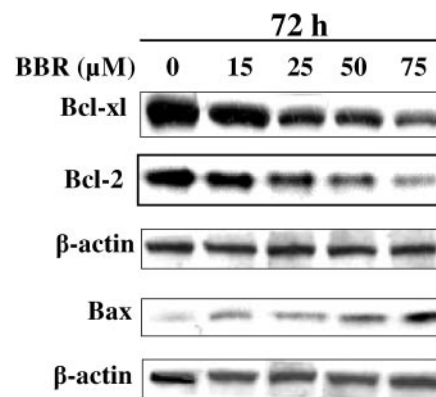
Fig. 5. Treatment of A431 cells with varying concentrations of berberine (0, 15, 25, 50 and 75 μM) for 72 h results in a dose-dependent reduction in the expression of the anti-apoptotic proteins Bcl-xl and Bcl-2, while increasing the expression of the pro-apoptotic protein Bax. After treatments for 72 h, cells were harvested, cell lysates prepared and subjected to western blot analysis to determine the expression of different proteins. β-actin was used to verify equal loading of the samples. BBR, berberine.
